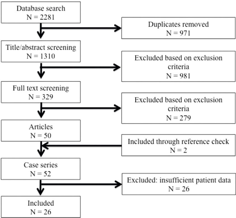
Figure 1. PRISMA-guided search.
